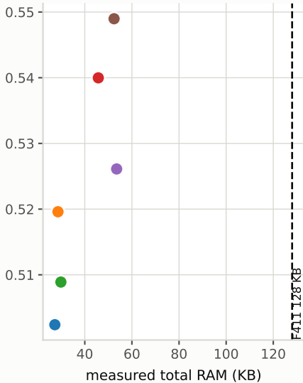
(b) accuracy vs peak SRAM
