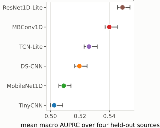
(b) mean AUPRC, record-level bootstrap 95% CI
