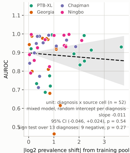
(c) no consistent association detected
