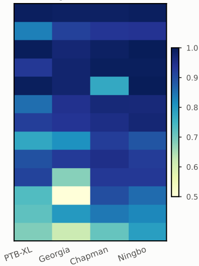
(b) diagnosis-level AUROC
