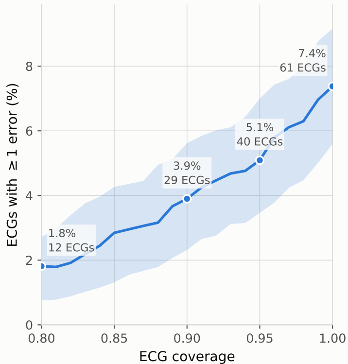
A Uncertainty-based referral of whole ECGs
