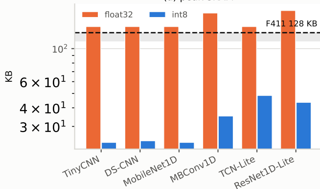
(a) peak SRAM
