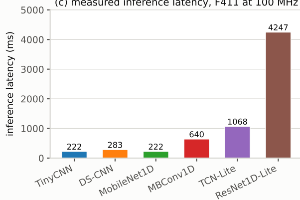
(c) measured inference latency, F411 at 100 MHz
