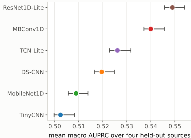
(b) mean AUPRC, record-level bootstrap 95% CI
