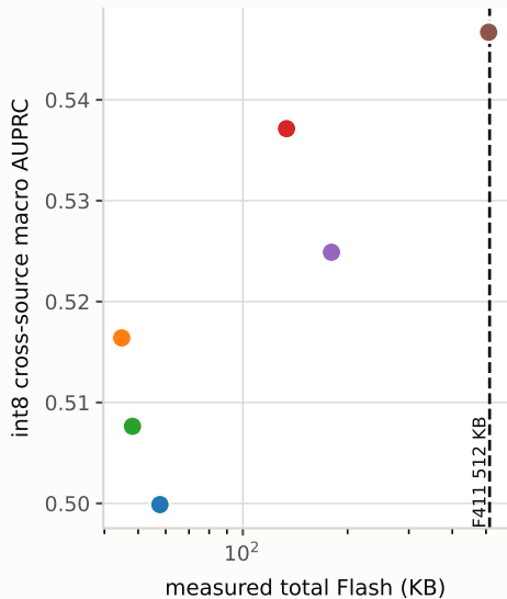
(a) int8 AUPRC vs Flash
