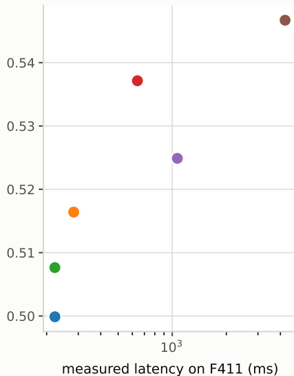
(c) int8 AUPRC vs measured latency
