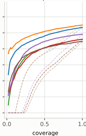
Chapman
