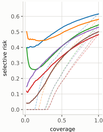
PTB-XL
