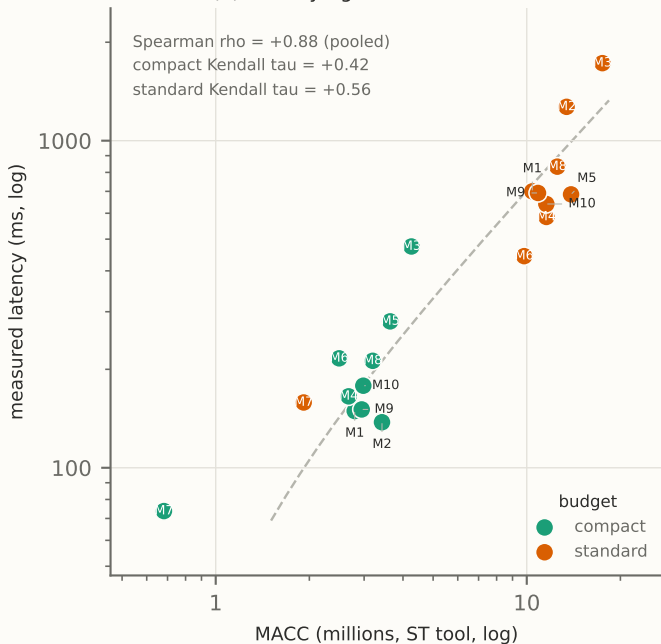
(a) latency against arithmetic cost
