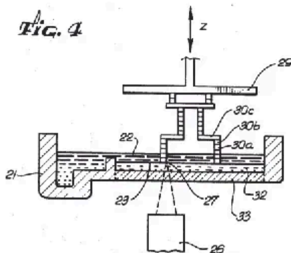
Figure 14.4: Here is an example of a schematic from Chuck Hull's 3-D printer patent provided by the US Patent and Trademark Office. (credit: modification of "US Patent US4575330A" by Charles W. Hull/Google Patents, Public Domain)
