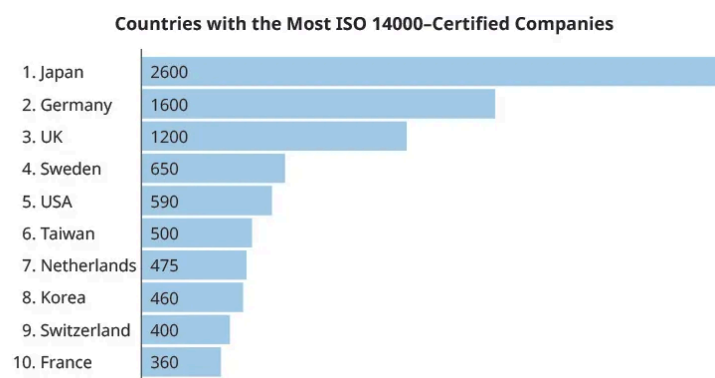
Quantitative = Data
