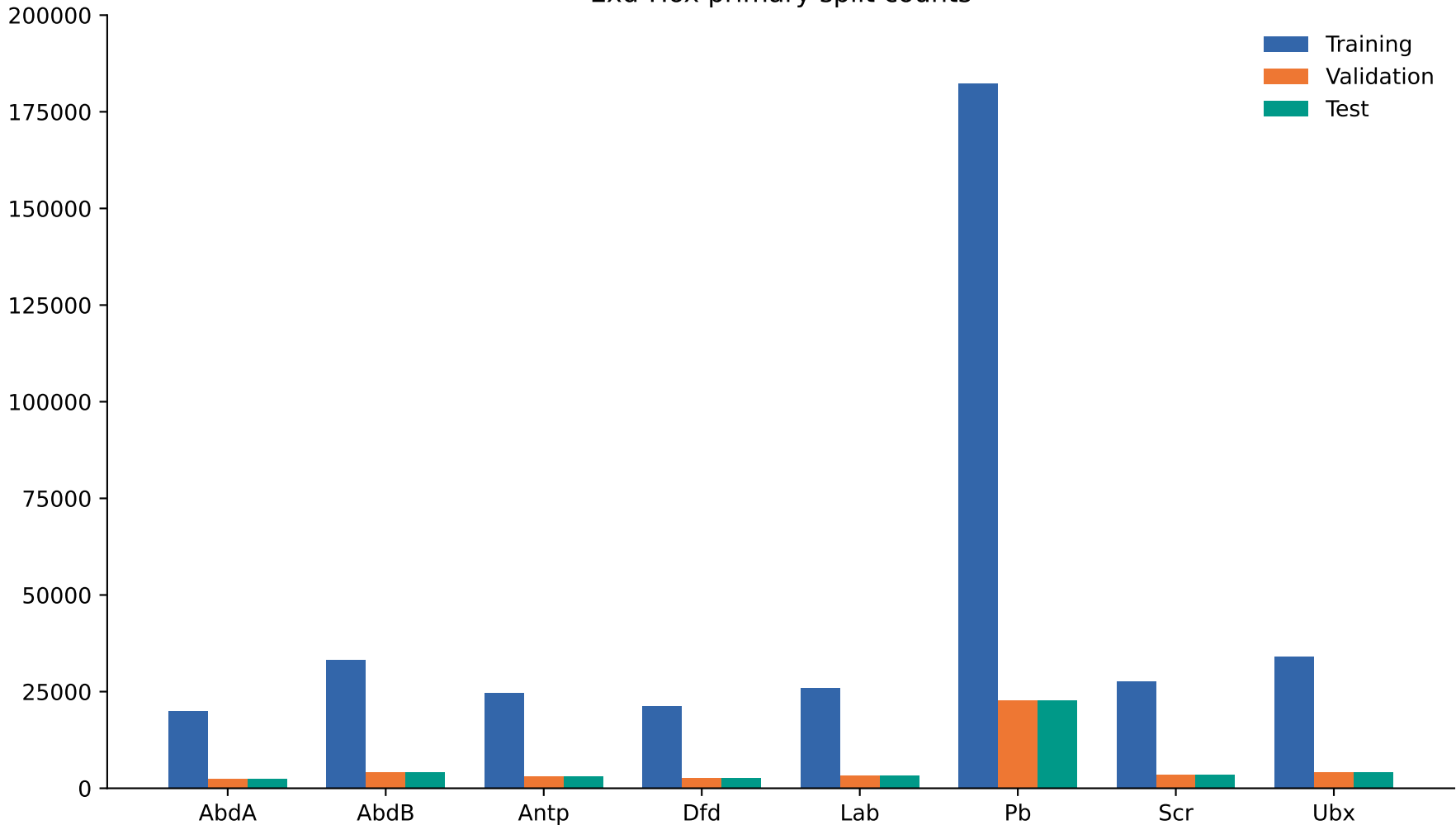
Exd-Hox primary split counts
