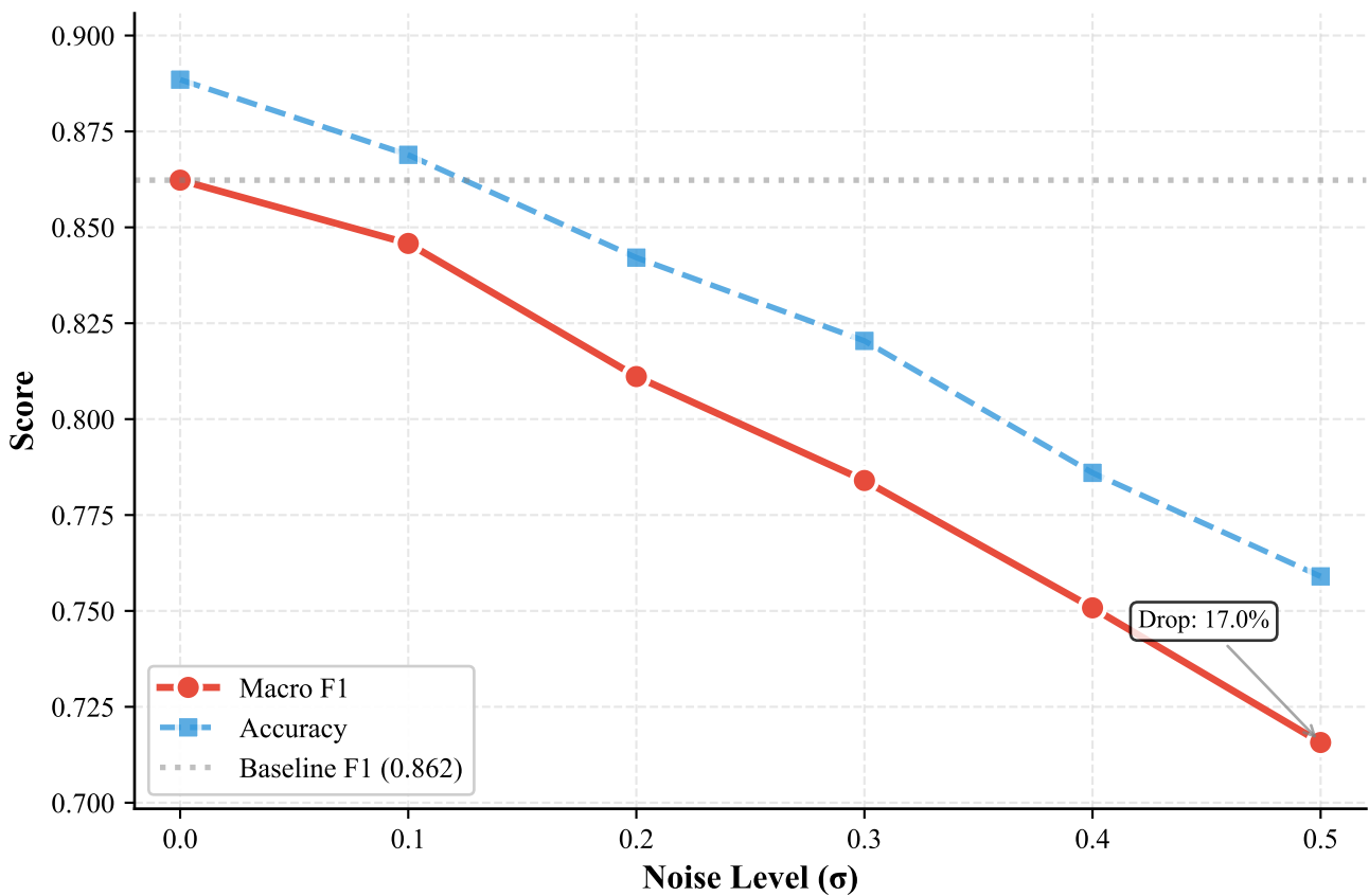
AMSNetV2 Noise Robustness
