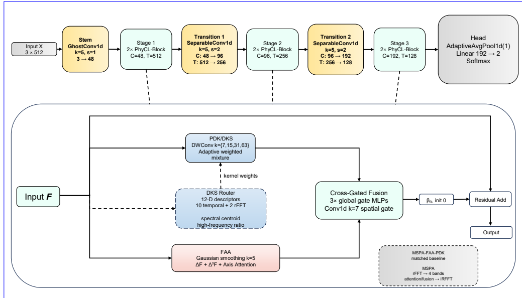
Figure 1: The overall architecture of PhyCL-Net. The Within each PhyCL-Block, the feature input signal is processed by two parallel branches: the Physics-Guided Dynamic Kernel (PDK) for adaptive receptive fields and the Fall-Aware Attention (FAA) for jerk-extractionsmoothed temporal-difference cues and axis attention , fused via the Cross-Gated Fusion Unit. The detailed internal structure of a single PhyCL-Block is also shown, illustrating the two parallel streams (PDK for multi-scale temporal adaptation and FAA for transient emphasis) and their integration through the symmetric cross-gated fusion unit. The proposed model has no active MSPA frequency-feature branch; the dashed path carries 10 temporal and two rFFT routing descriptors. FAA retains Gaussian smoothing ( k = 5 ), first and second differences, and axis attention; fusion uses three global gate MLPs and a k = 7 spatial gate before the scaled residual addition.
