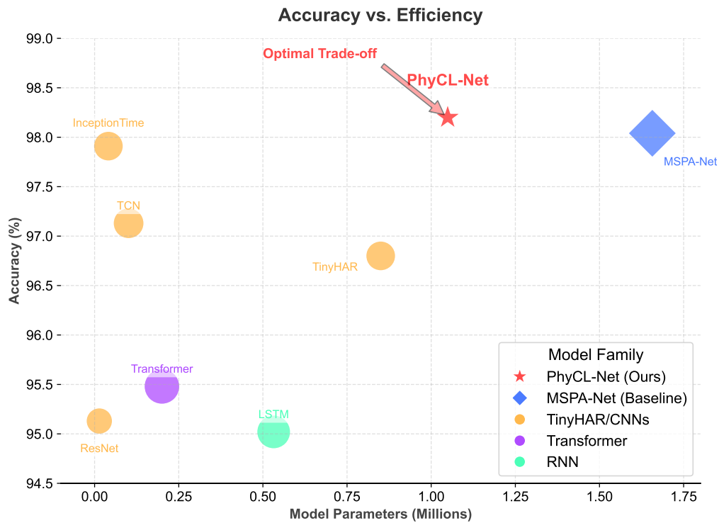
Figure 3: Accuracy-efficiency trade-off. Bubble size is proportional to single-thread CPU latency (p50). PhyCL-Net (red star) achieves has the best highest reported accuracy (98.21%) while maintaining a competitive parameter count (among the models in Table 2, with 1.049M )-parameters and low latency (125.99 ms )median latency. The plot label MSPA-Net denotes MSPA-FAA-PDK. The additional TinyHAR point is retained from the supplied figure and is excluded from the manuscript’s quantitative comparisons.
