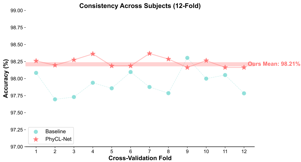
Figure 4: Cross-validation stability analysis. The fold-wise Fold-wise performance comparison across 12 subjects demonstrates that PhyCL-Net consistently outperforms the matched spectral baseline in almost every fold. This is a descriptive comparison, exhibiting lower not a test of variance and higher stability reduction or statistical superiority.
