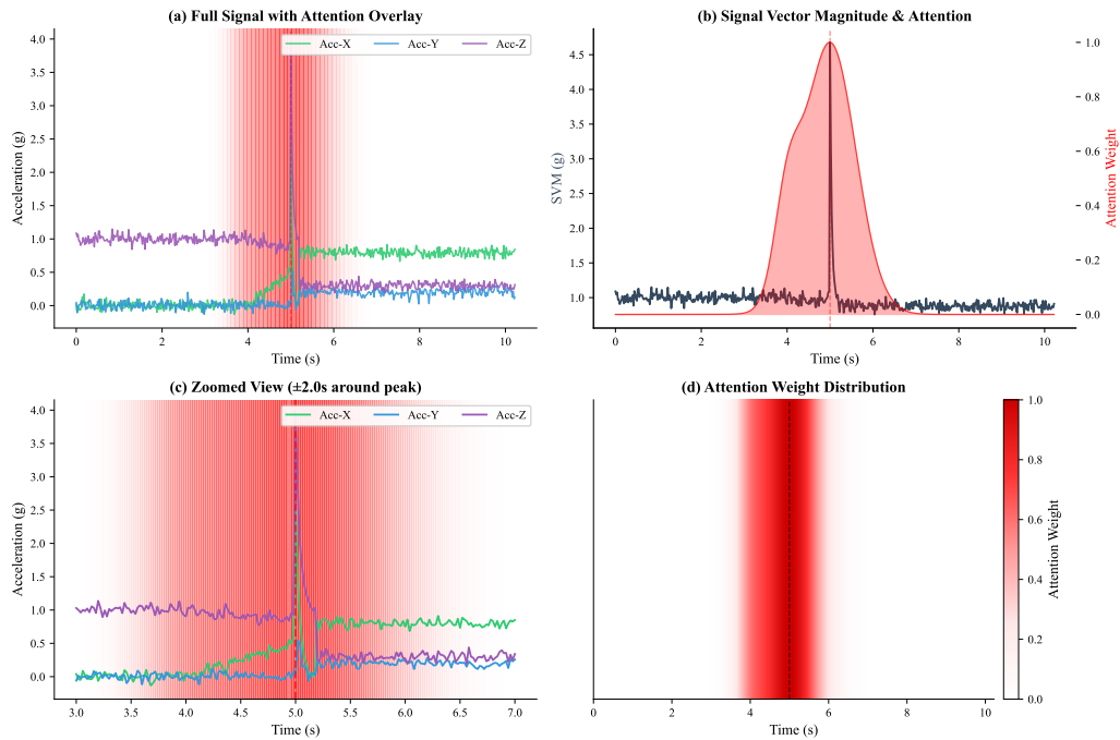
Figure 7: Attention visualization of the Fall-Aware Attention (FAA) module. The attention weights highlight jerk-dominant segments corresponding to impact phases, demonstrating the module's ability to focus on kinematically relevant regions display illustrates temporal emphasis near impact-like transients; it does not independently establish physical jerk alignment or a causal performance contribution.
