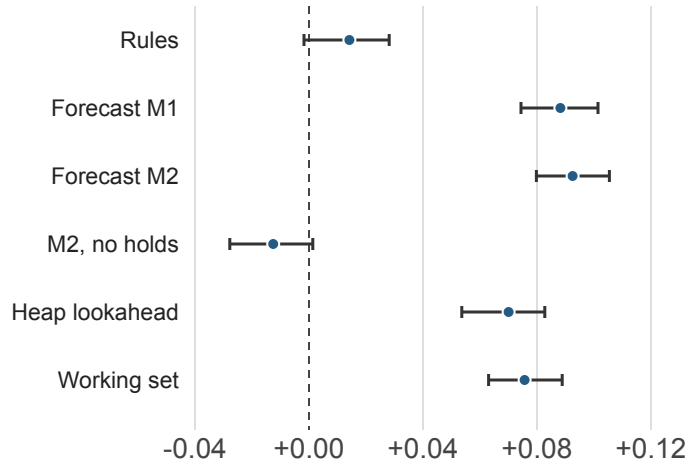
Interactive SLO difference
