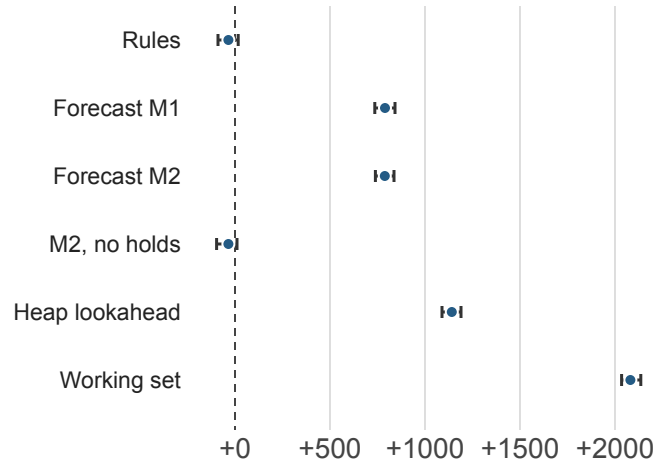
Background JCT difference (s)
