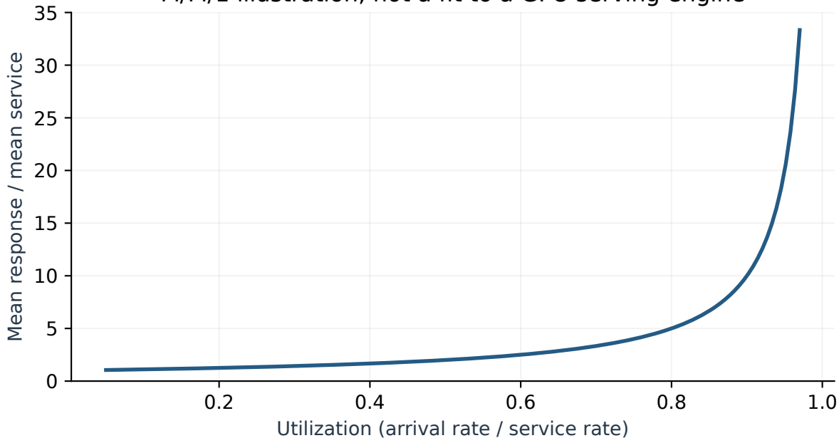
M/M/1 illustration; not a fit to a GPU serving engine
