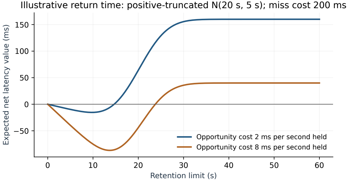
Figure 9: Derived retention value under two assumed memory opportunity costs. The return distribution is a normal distribution truncated to positive time. The miss penalty is 200 ms. The illustration shows that a forecast alone does not determine a retention policy; congestion changes the value of memory.
