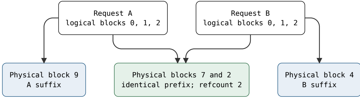
Figure 3: Logical-to-physical cache mapping. The first two logical blocks are shared; suffix blocks are private. Physical IDs need not be contiguous. An extension that would modify shared state requires safe ownership handling.
