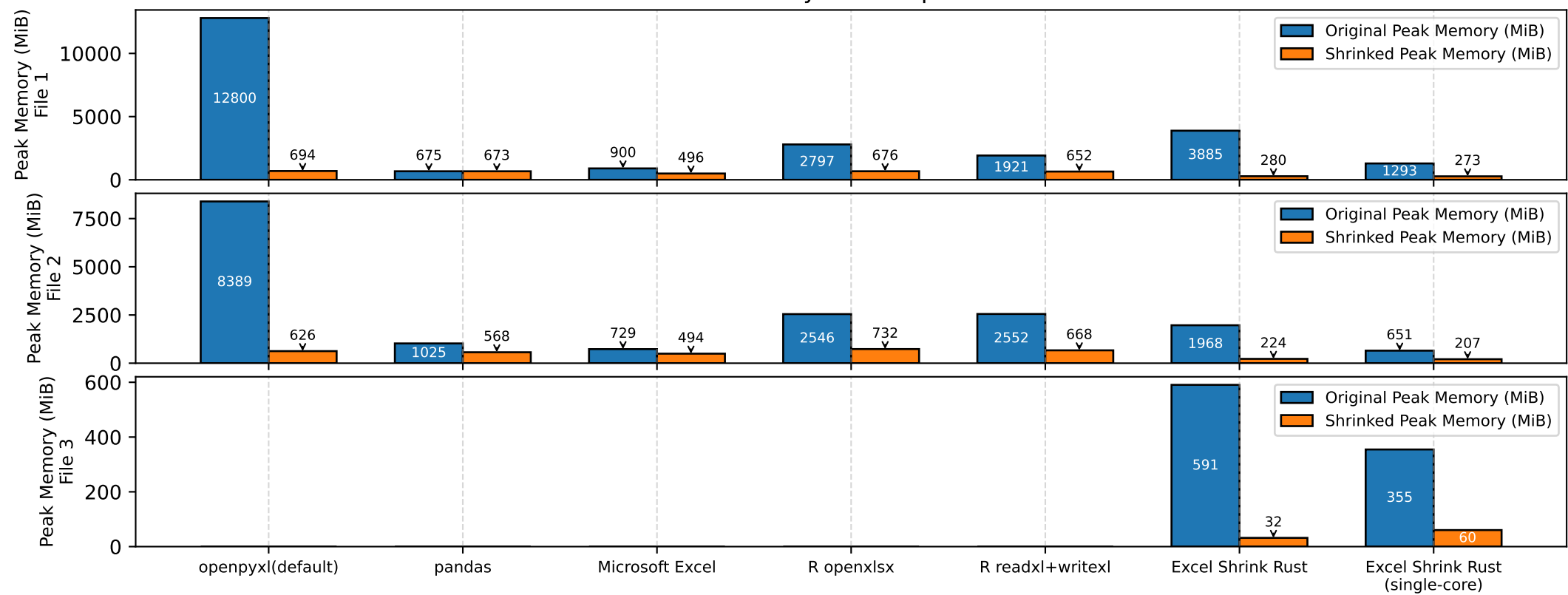
Memory Consumption
