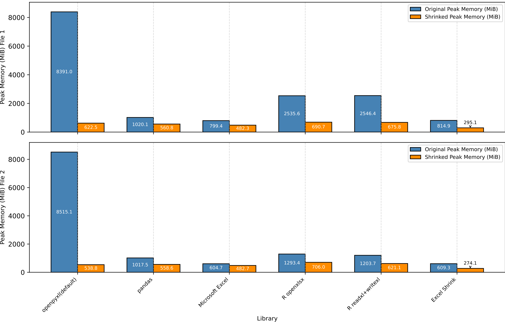
Memory Consumption
