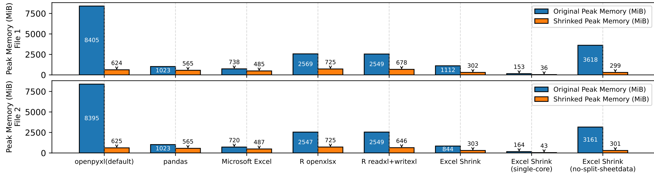
Memory Consumption
