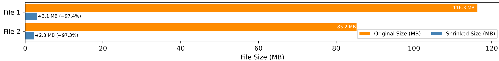
Memory Consumption
