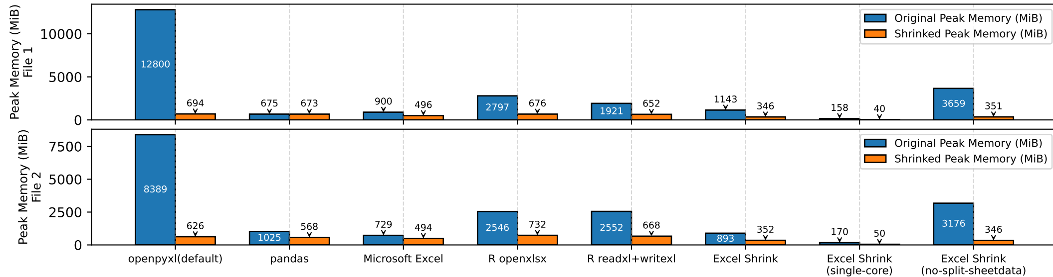
Memory Consumption
