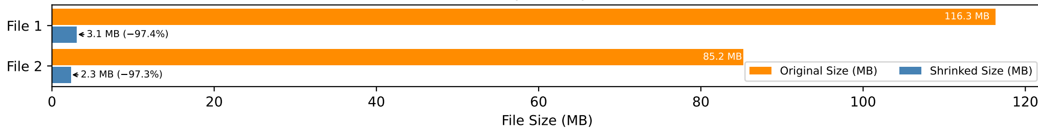
Memory Consumption
