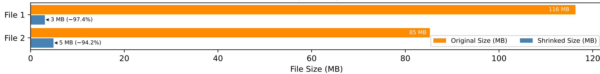
Memory Consumption
