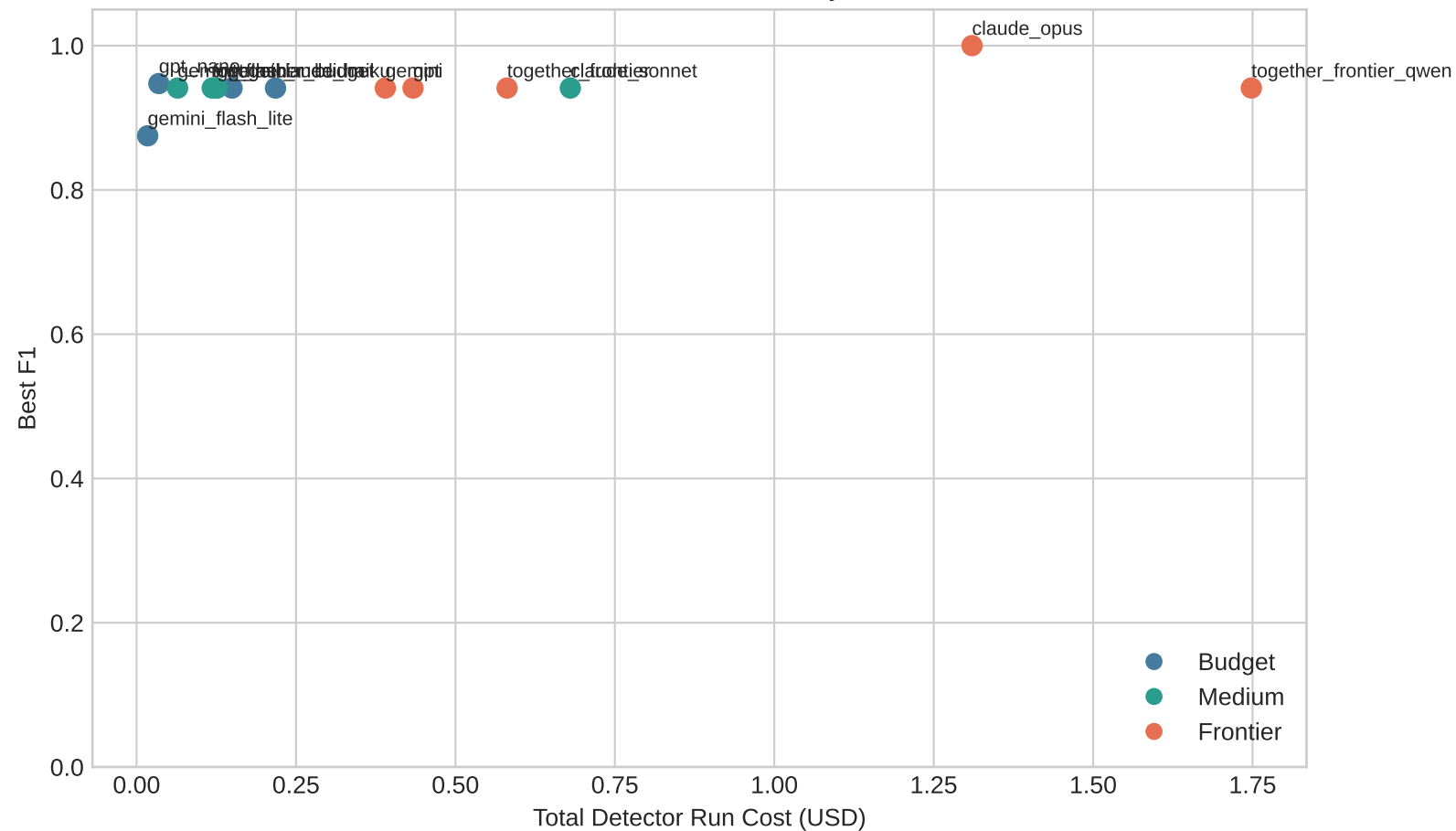
Cost / Performance Tradeoff by Detector
