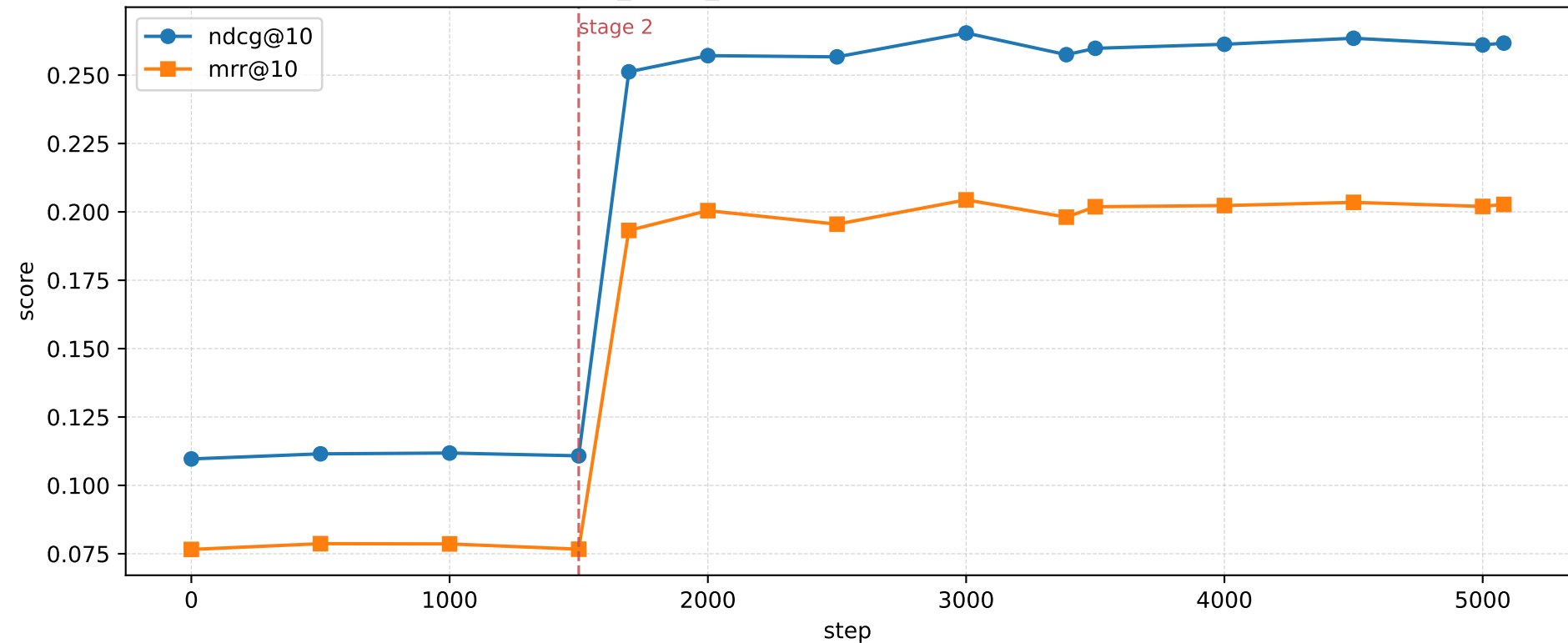
E11 per_token_gated — BEIR probe (in-validation)
