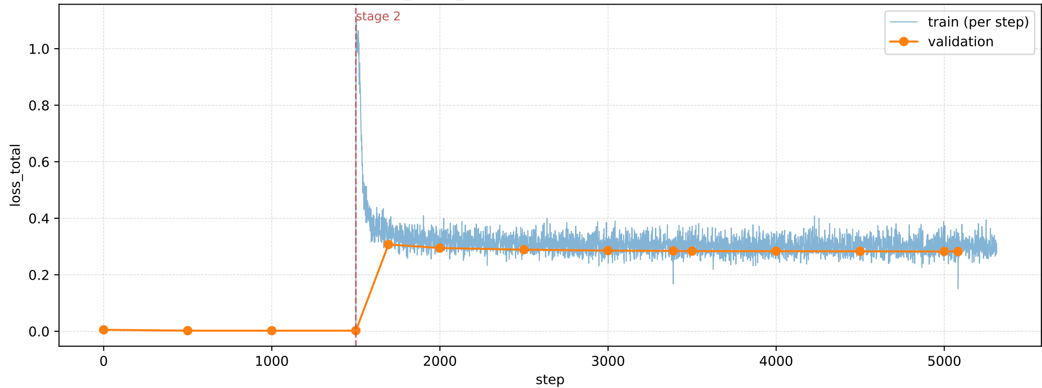
E11 per_token_gated — train vs validation total loss
