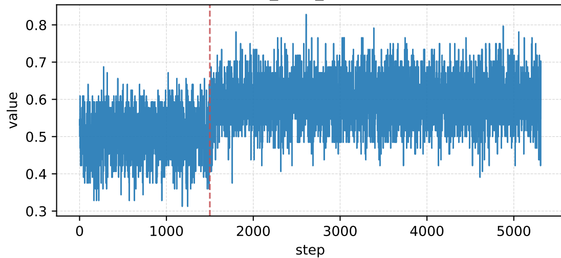
teacher_top1_agreement
