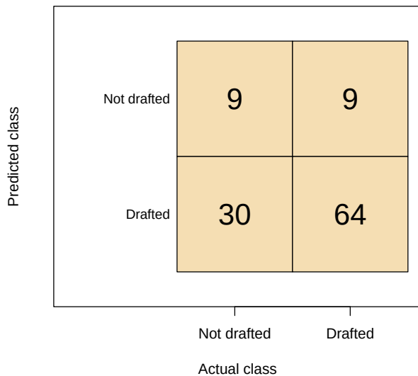
Confusion matrix
