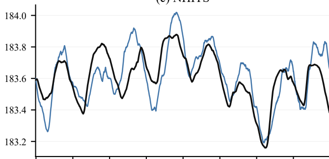
(c) NHITS
