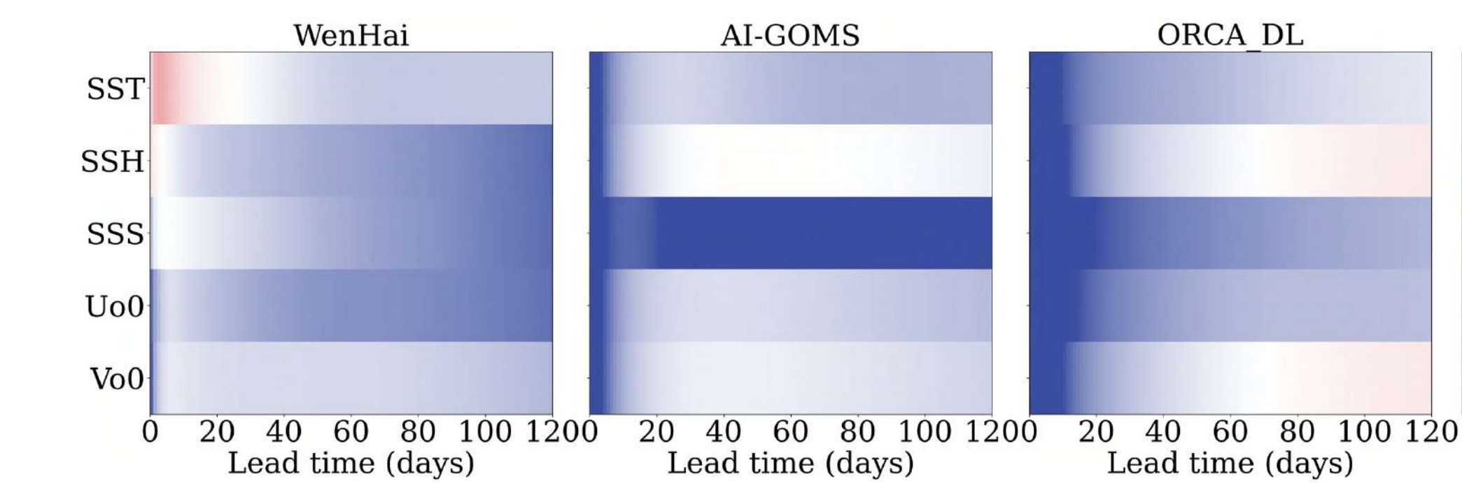
Scorecard for Global Ocean Simulation (RMSE Skill Score, 240 ICs)
