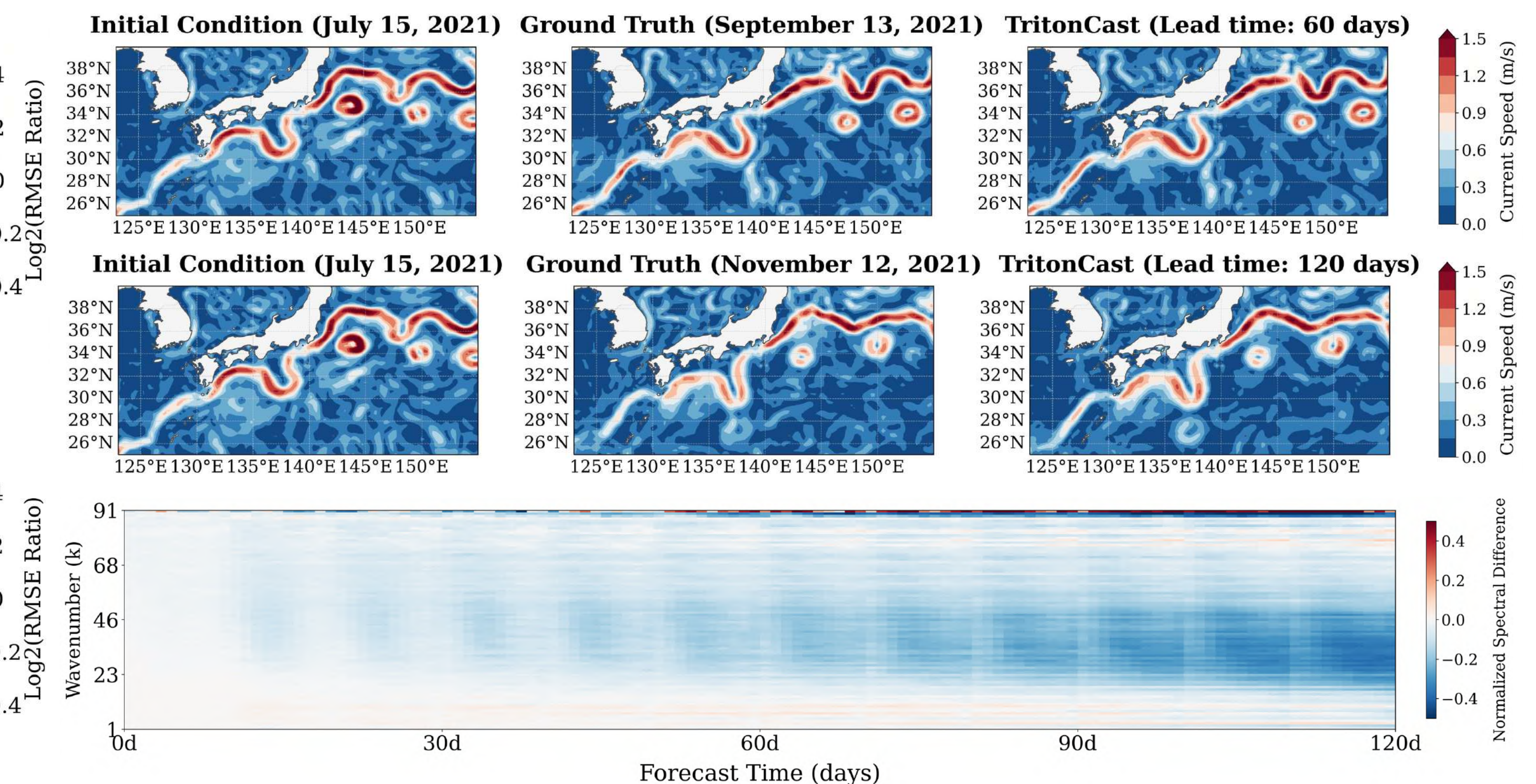
d Capture the Generation and Dissipation Process of Ocean Eddies.
