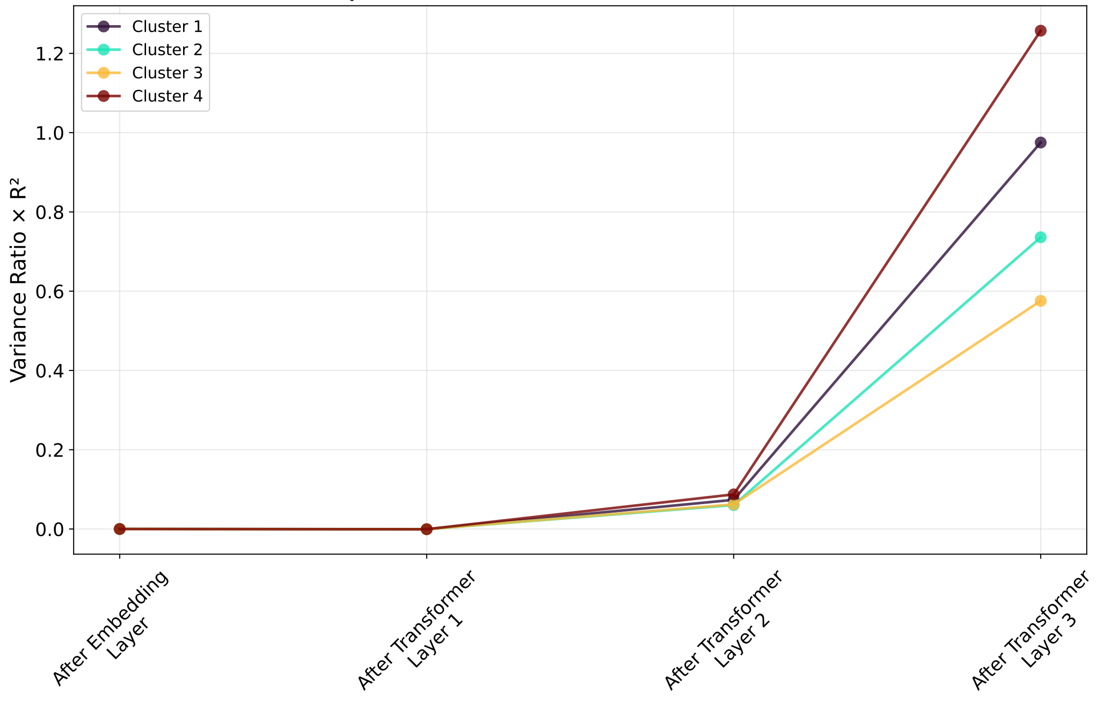
QM9 - Cluster Variance Ratio \times Global R^2
