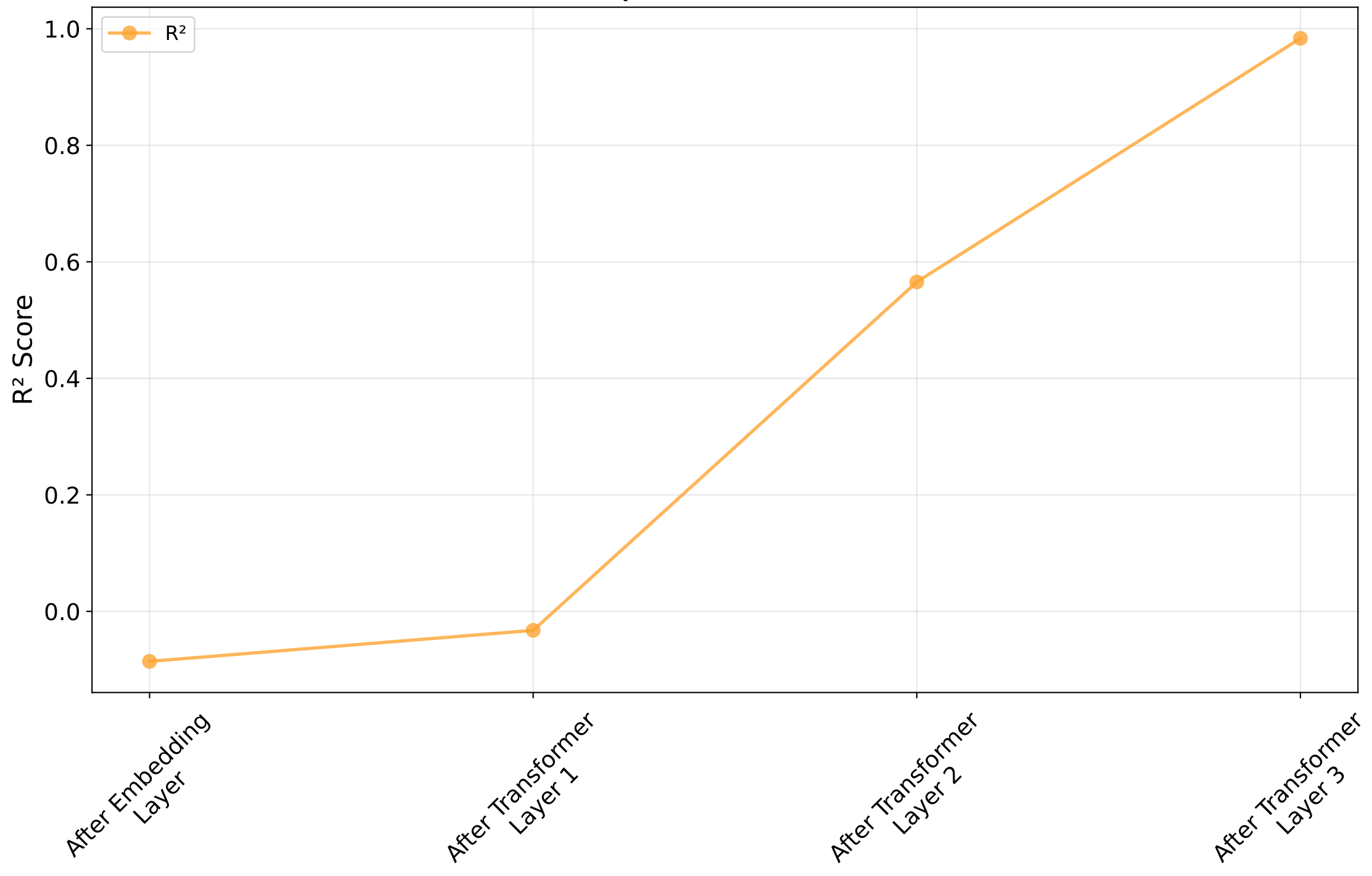
QM9 - Global R^2
