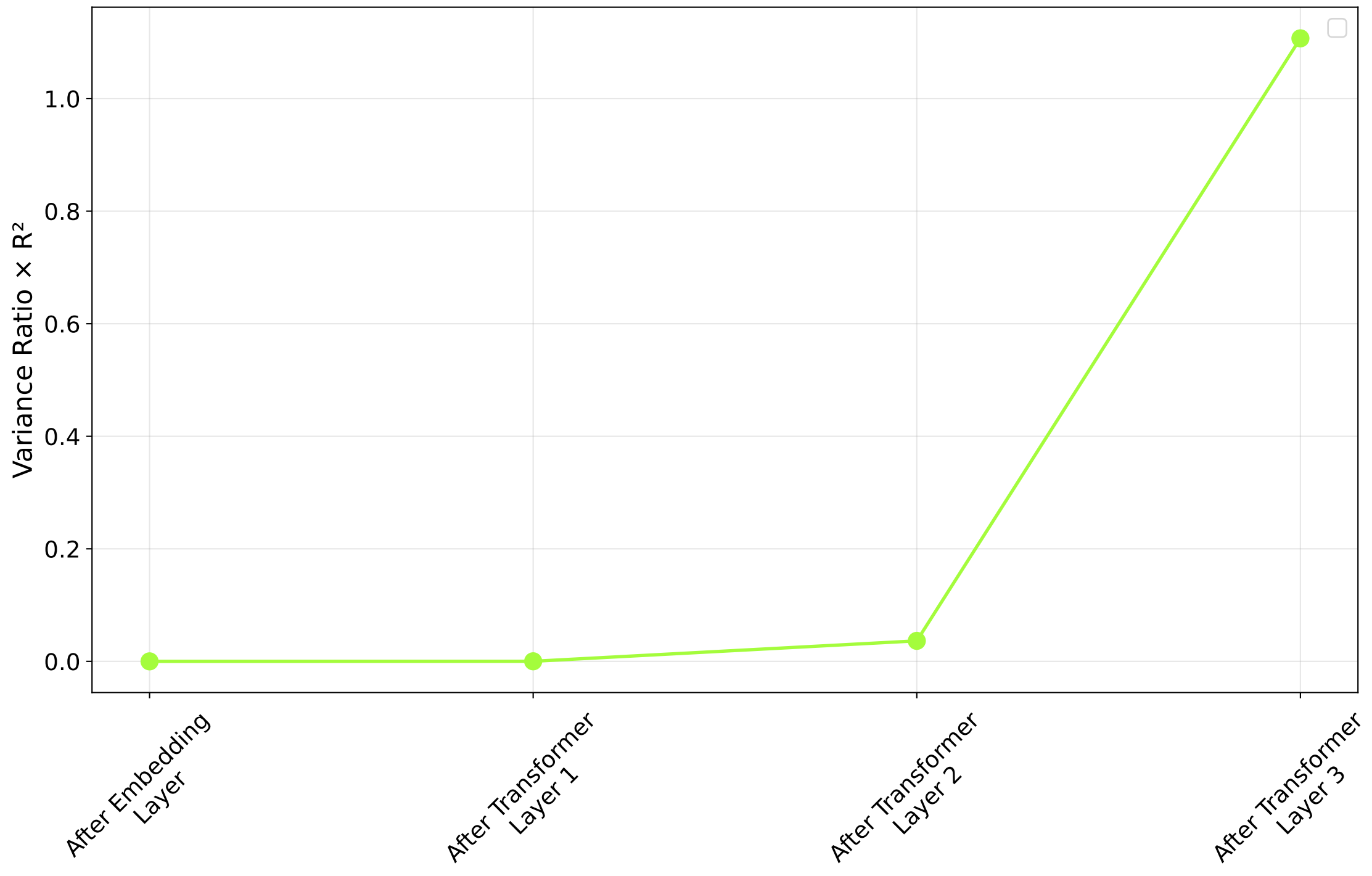
HCE - Variance Ratio \times R^2
