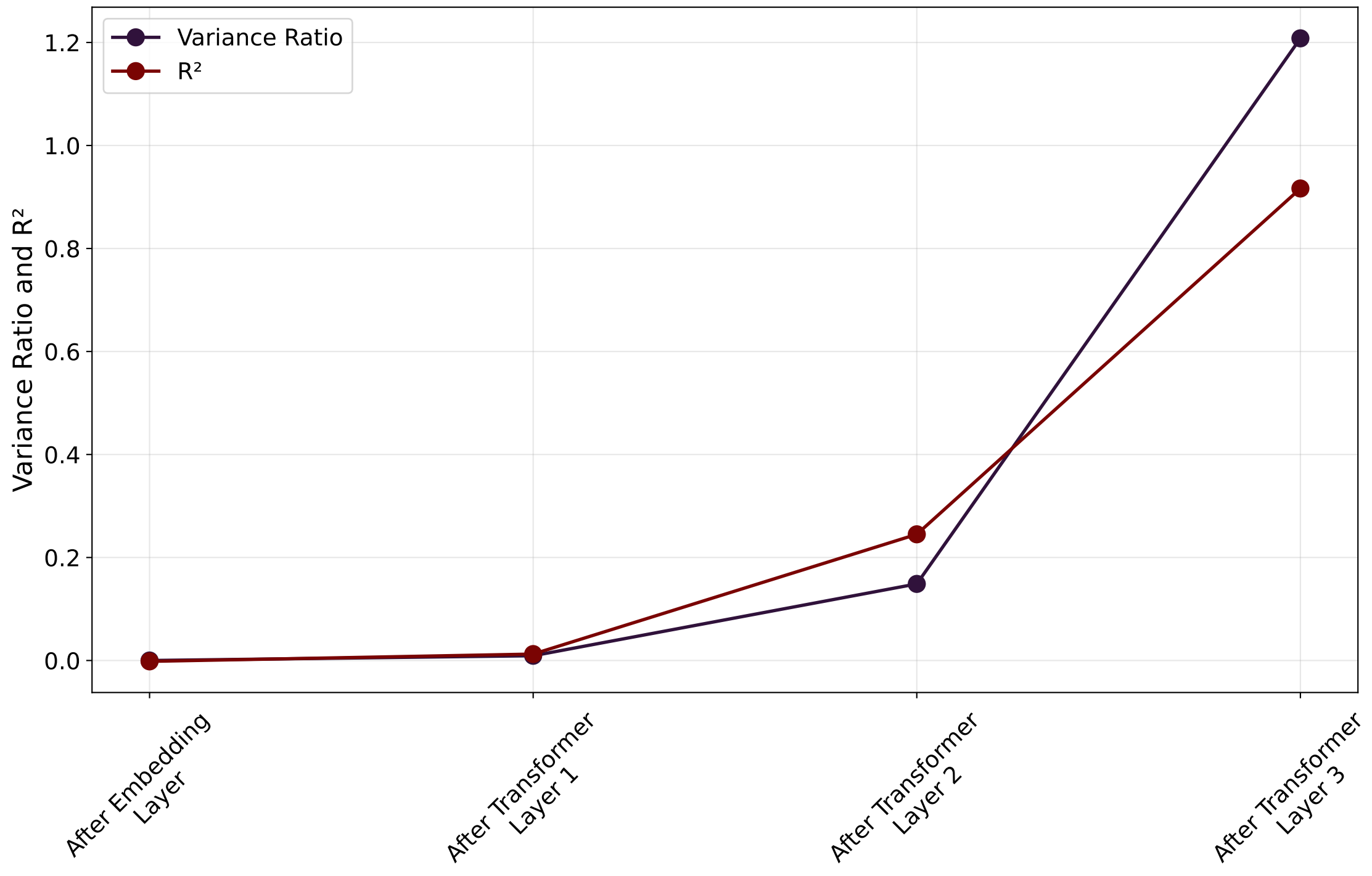
HCE - Variance ratio and R^2
