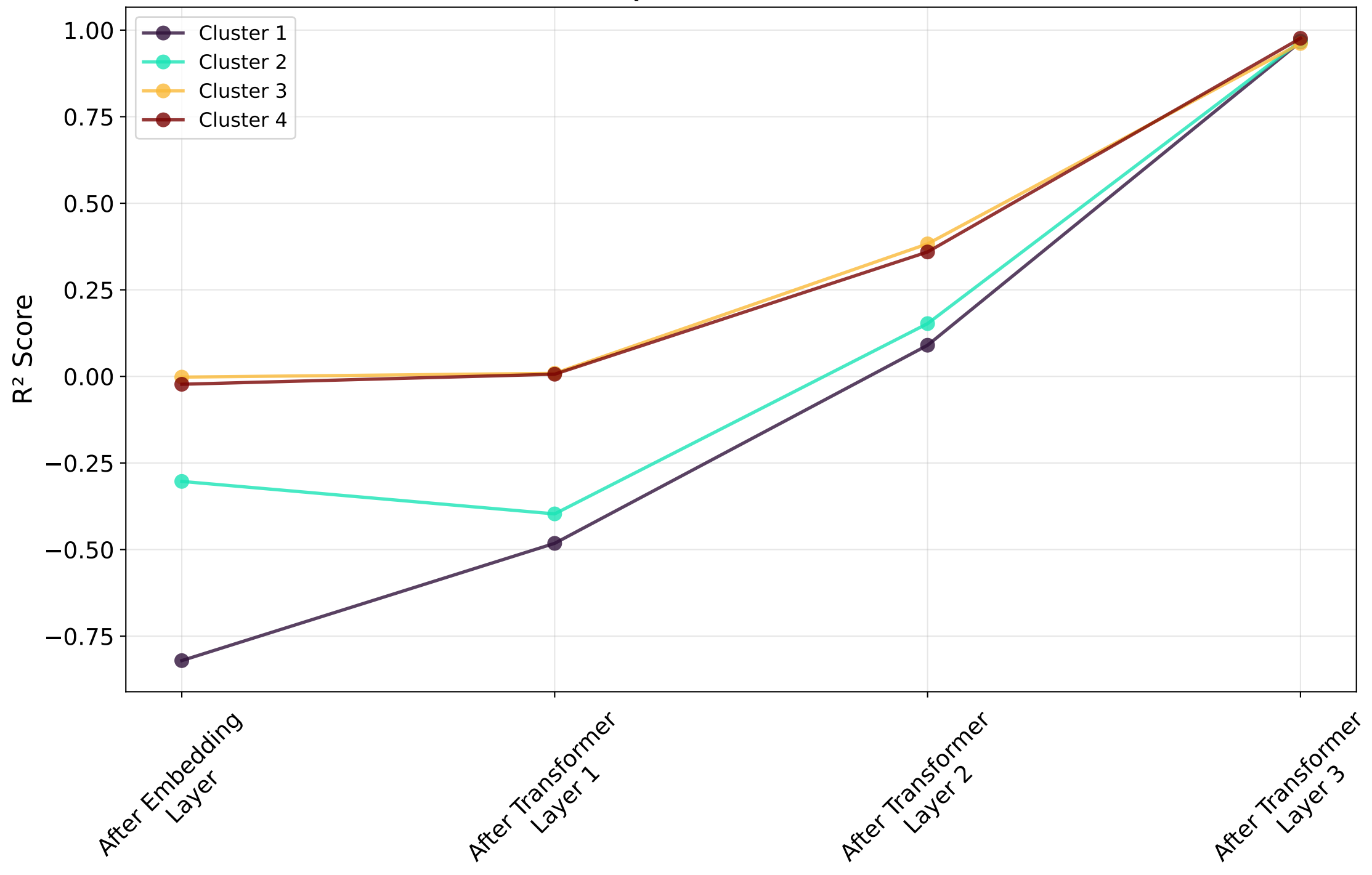
QM9 - Cluster R 2
