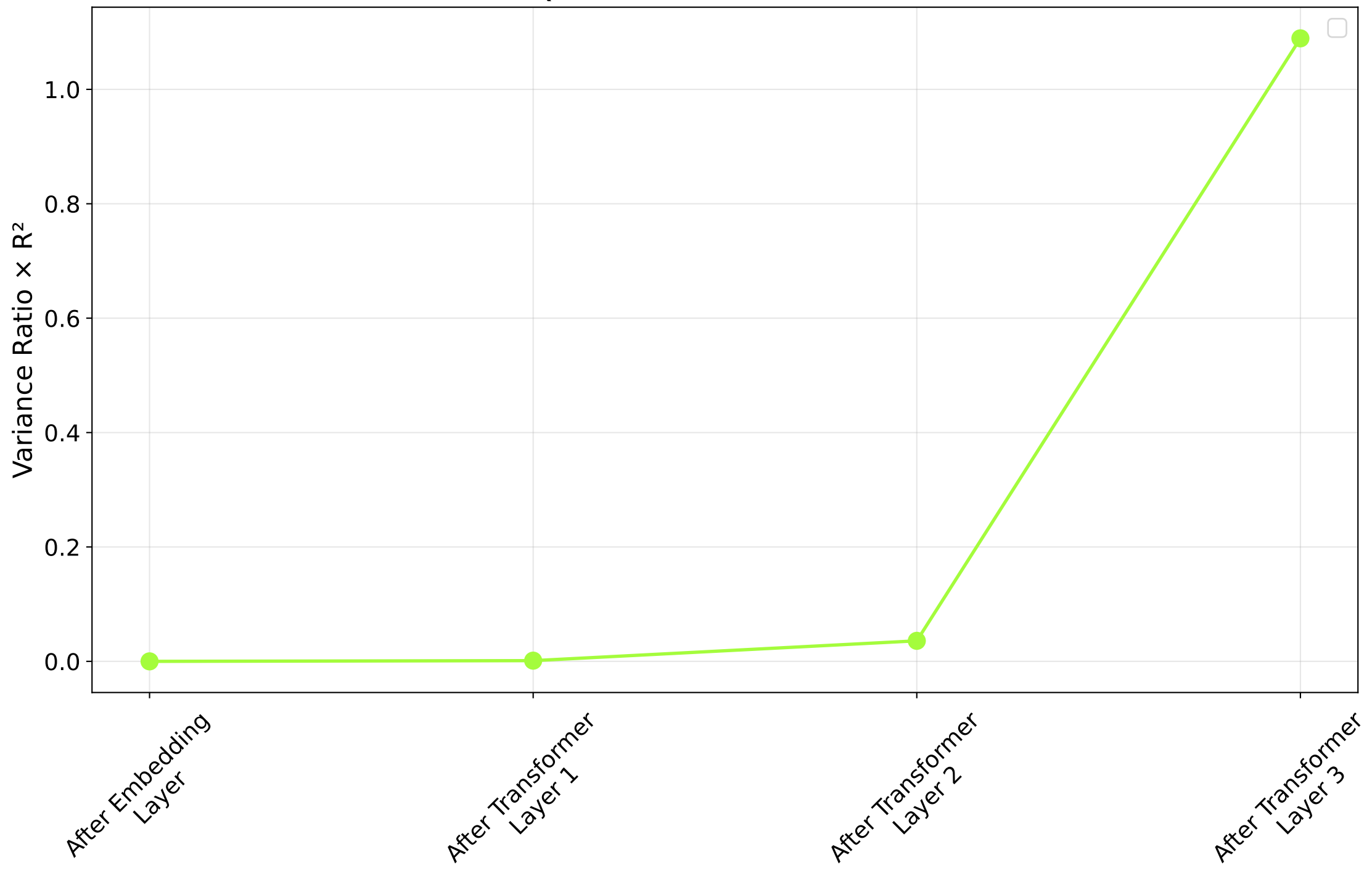
QM9 - Variance Ratio \times R^2
