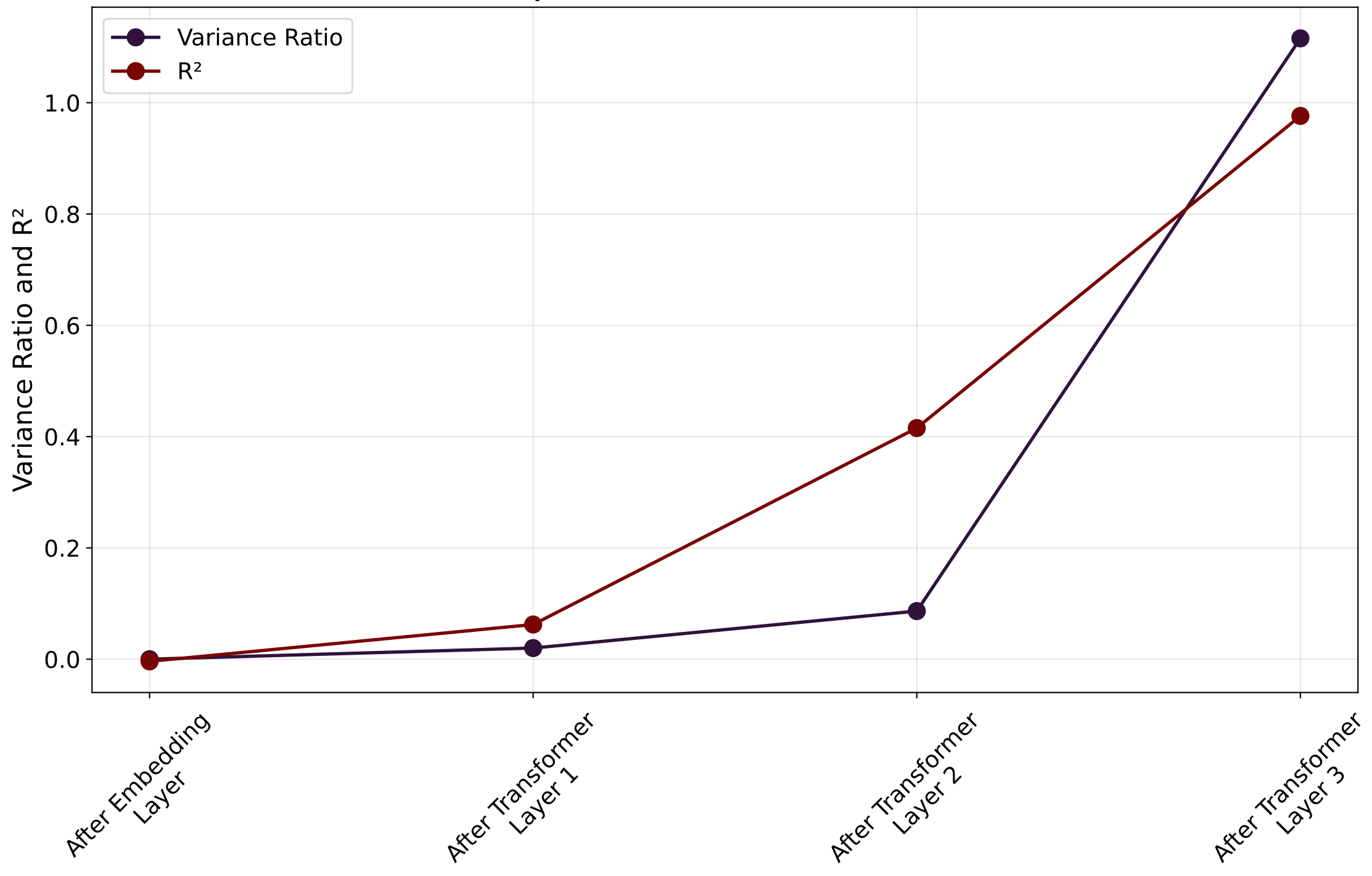
QM9 - Variance ratio and R^2
