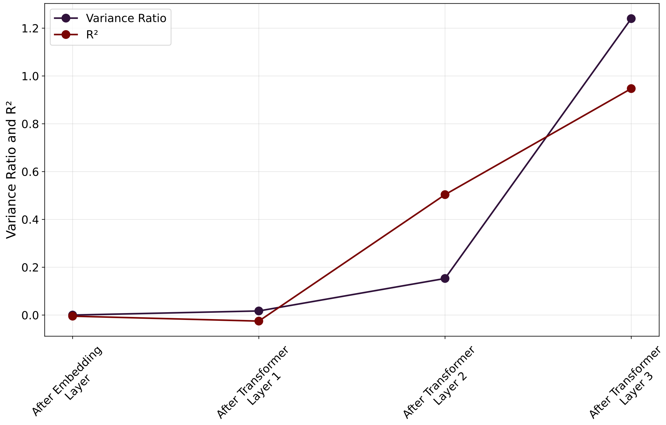
ESOL - Variance and R^2
