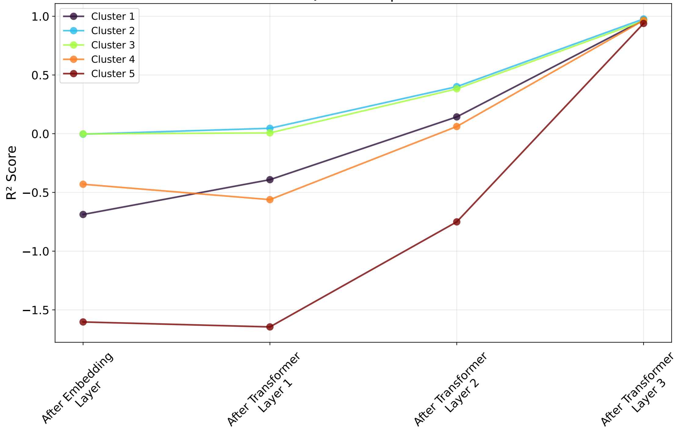
QM9 - Group R^2
