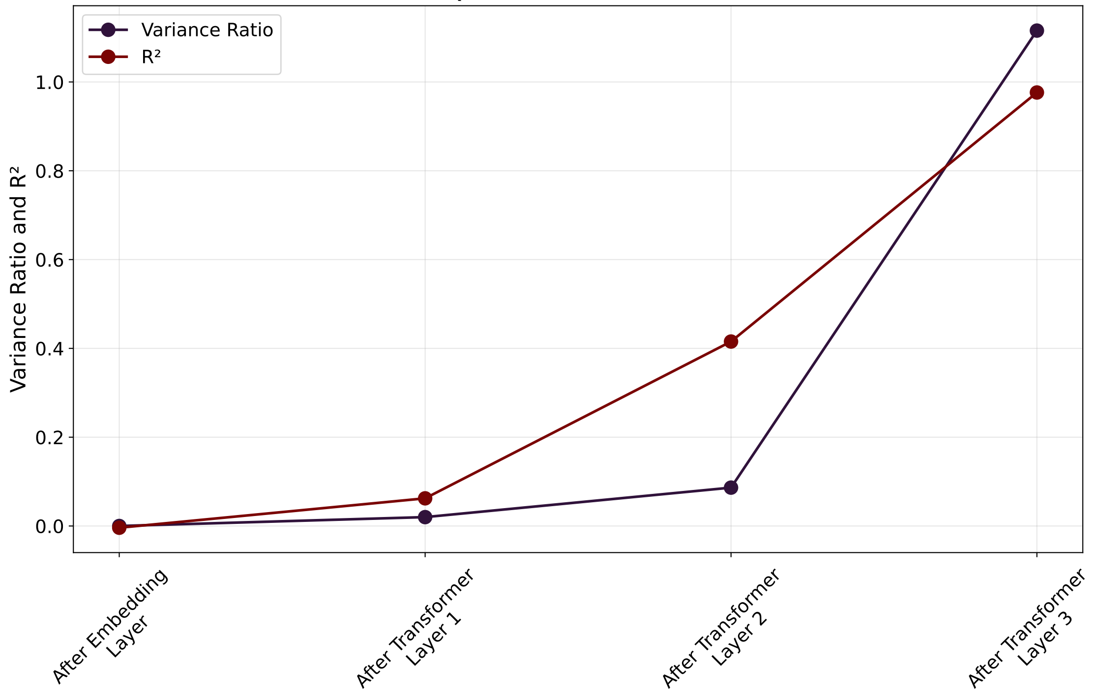
QM9 - Variance and R^2
