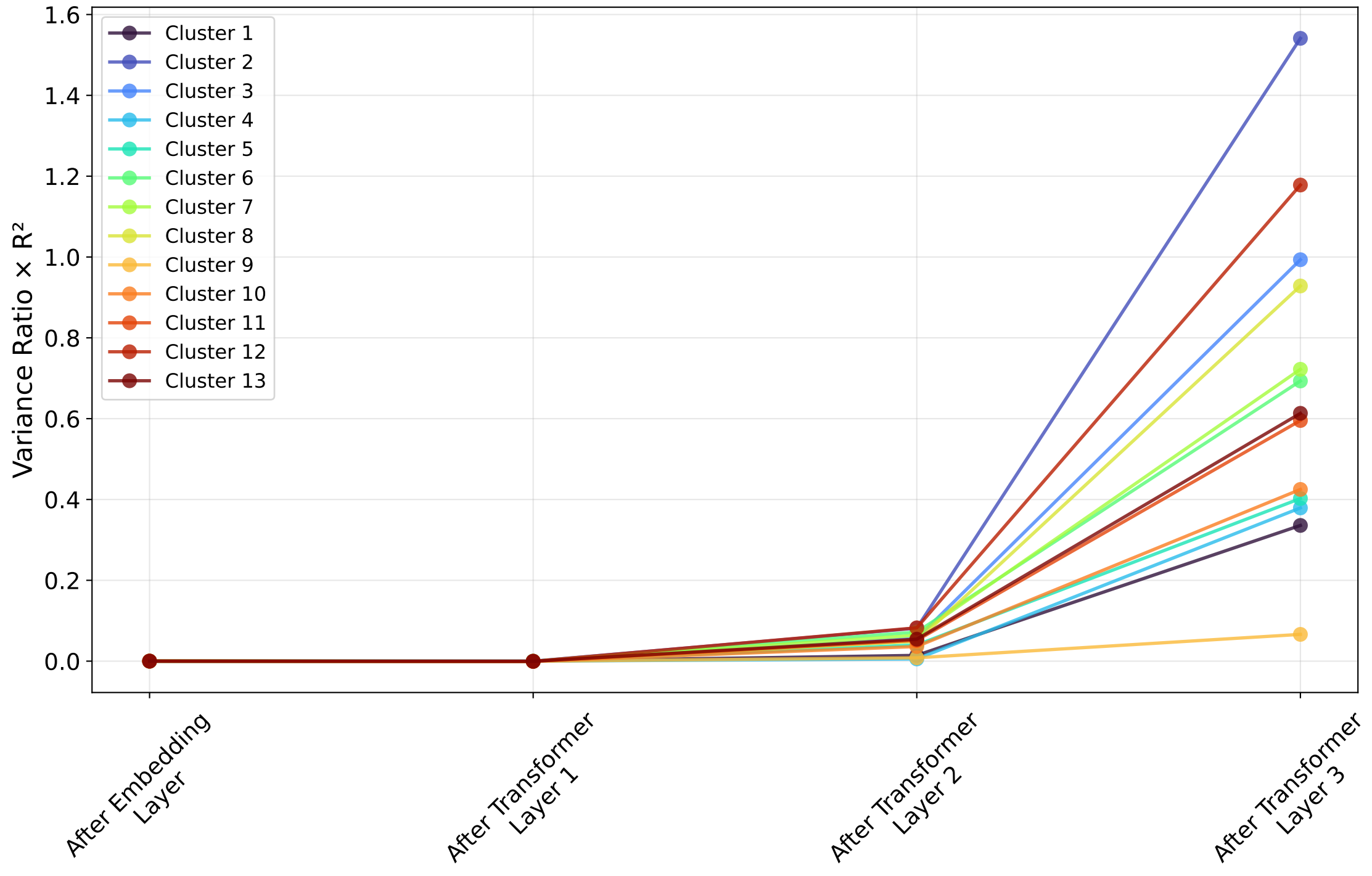
ESOL - Cluster Variance Ratio \times Global R^2
