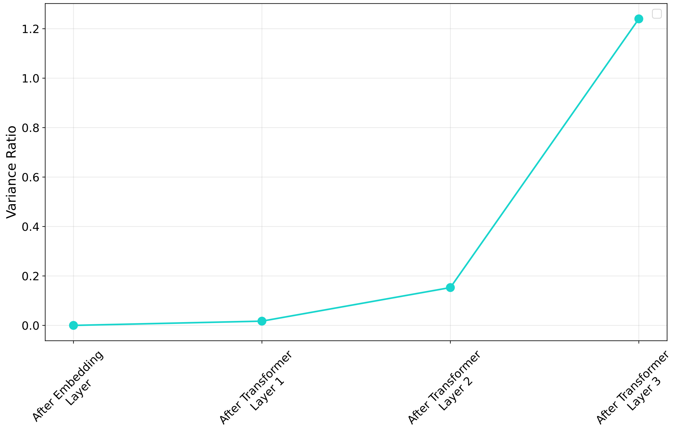
ESOL - Variance Ratio
