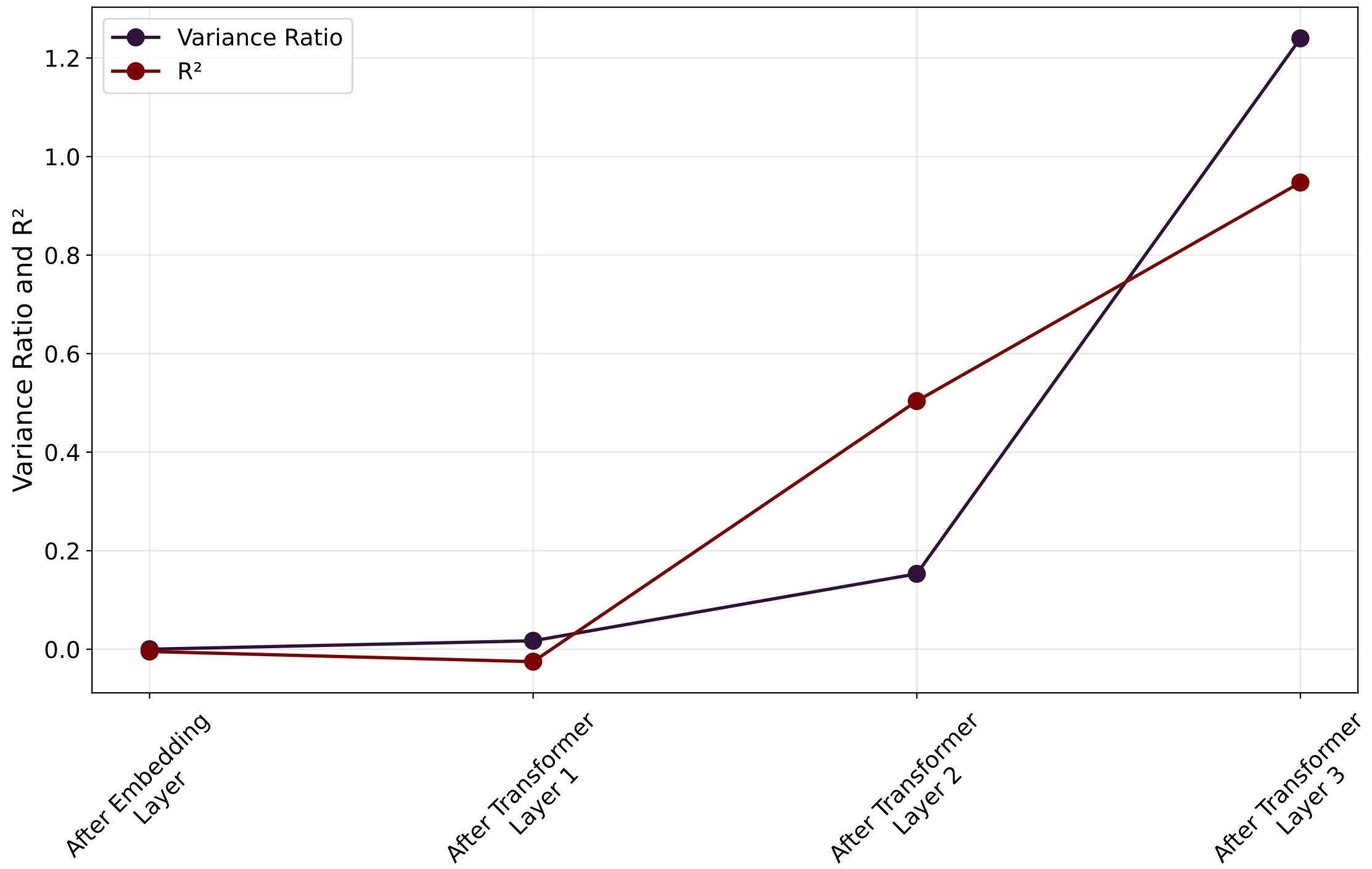
ESOL - Variance ratio and R^2
