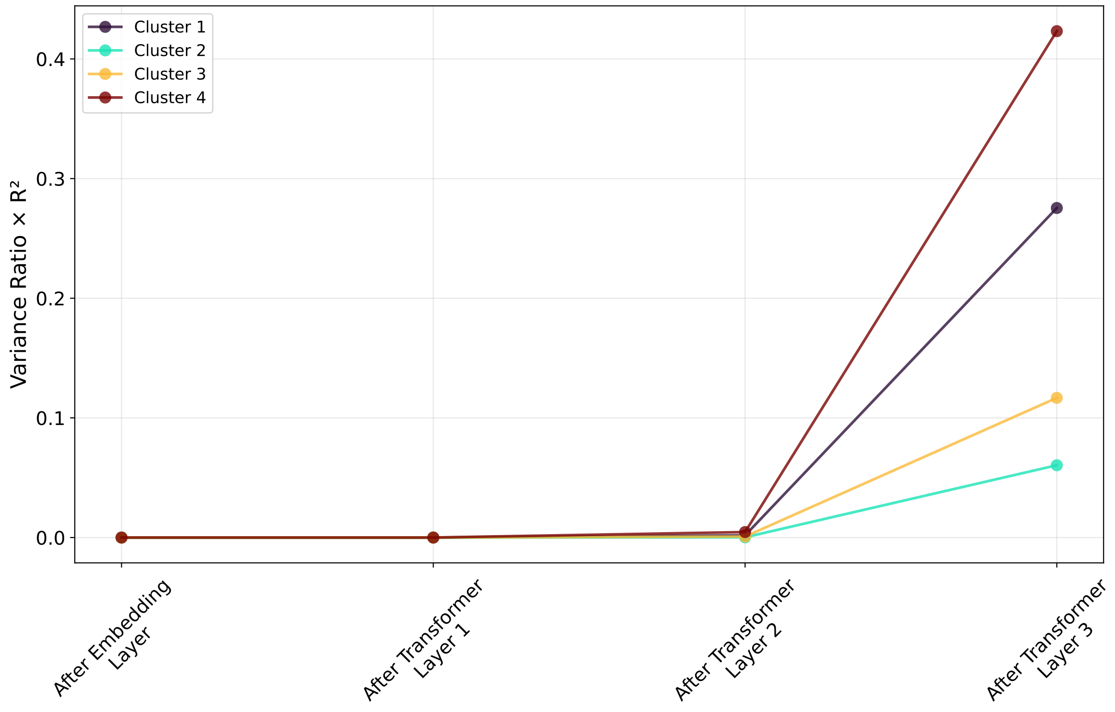
HCE - Cluster Variance Ratio \times Global R^2
