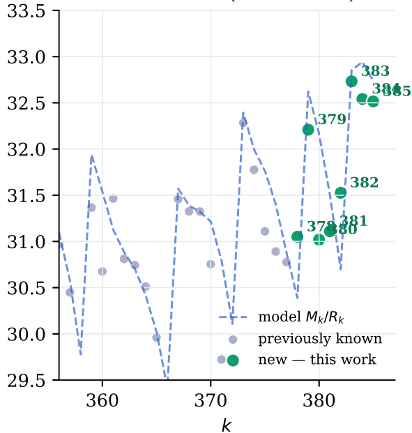
frontier detail ( k = 356-385 )
