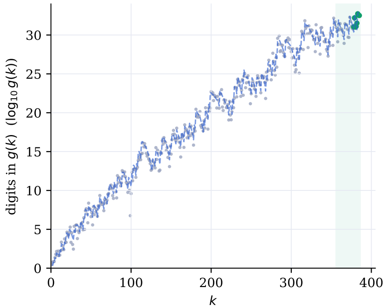
all 385 terms
