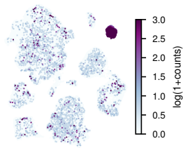
b tryptase/CPA3
