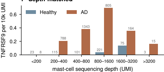
f depth-matched
