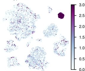
b tryptase / CPA3
