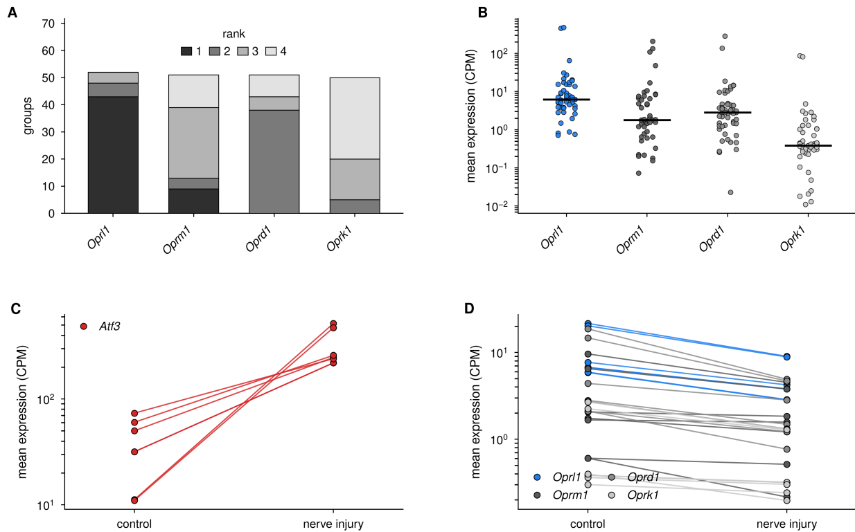
Figure 3. The four opioid receptor genes in bulk RNA-seq of ganglion tissue
