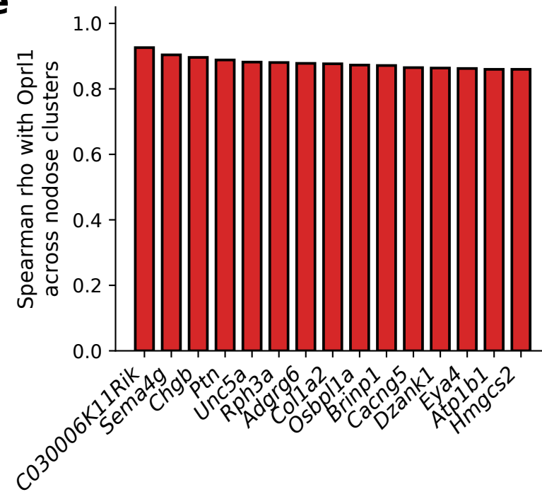
Top transcriptome-wide correlates (n = 21 clusters, 16,380 genes tested)
