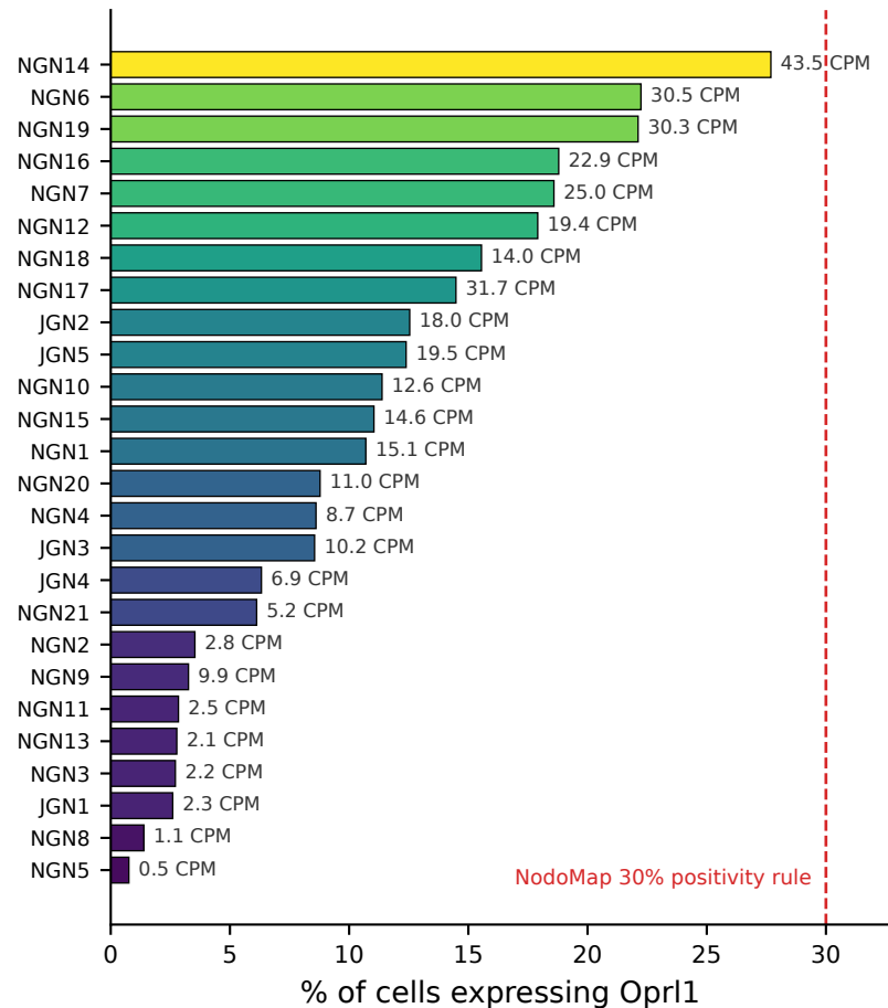
(B) Oprl1 across the 26 neuronal clusters nodose (NGN) and jugular (JGN)
