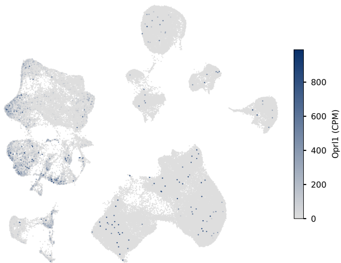
(A) Oprl1 on the published Nodemap UMAP 106,436 cells
