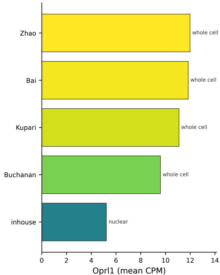
(C) Oprl1 by constituent dataset
